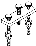
2200205 DRUM PULL TOOL 2321
