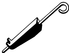
2108493 EXTRACTOR, TAPE PIN, AMP 380305-2
